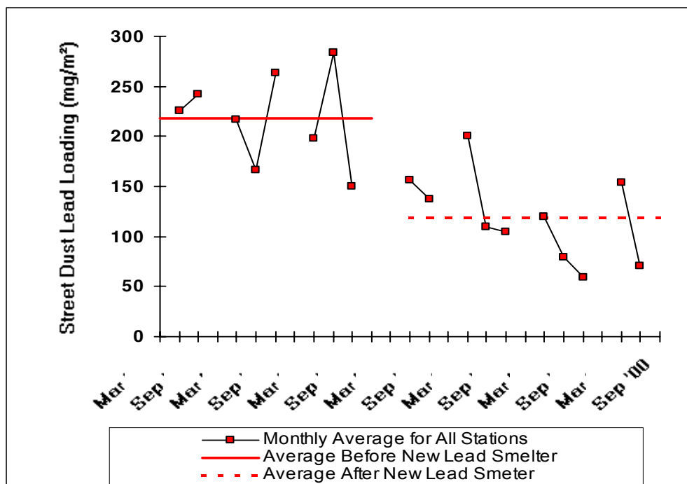
Figure 14 - Street Dust Lead Loadings Before/After New Smelter
