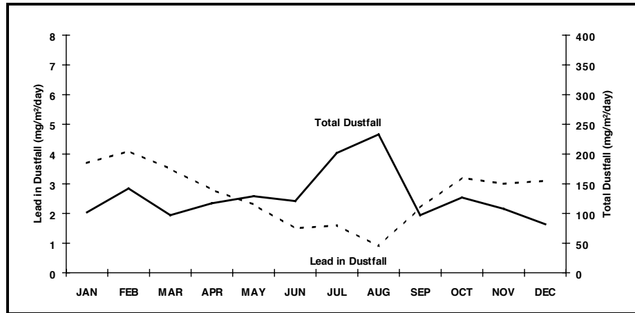
Figure 10 - Monthly Average Dustfall at Butler Park, 1975-1987
