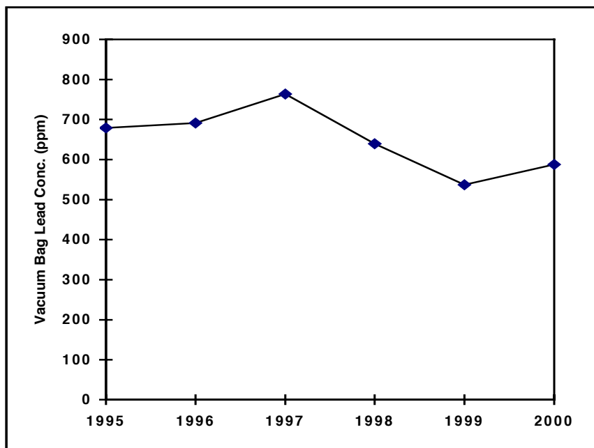
Figure 18 - Floor Dust Lead Concentrations by HEPA Vac
