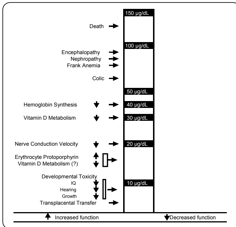
Figure 6 - Lowest Observed Effect Levels of Lead in Children
